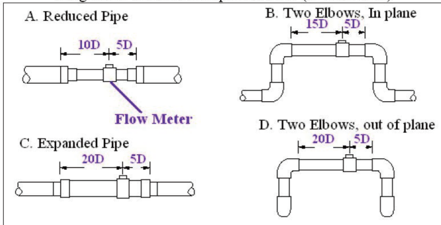
Diagram 2. Number of Pipe Diameter (D=Diameter)
