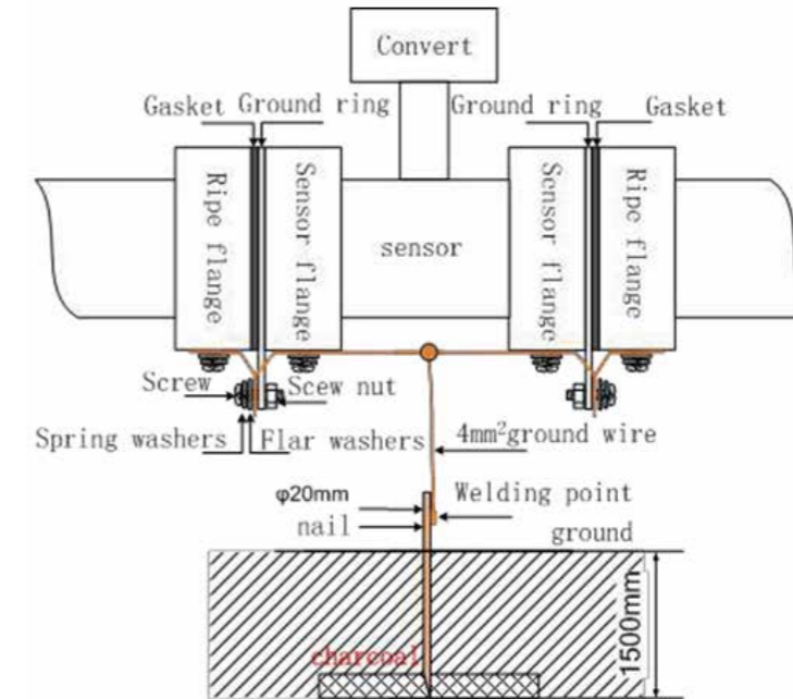
Fig.4.4(f) Grounding
