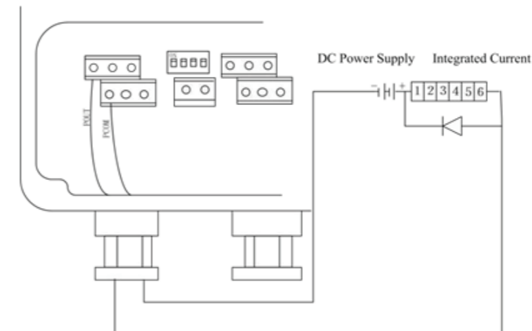
Fig.4.4 (b) Connection of electro-magnet counter
