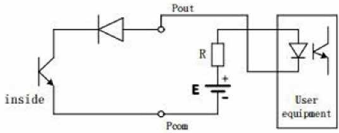
Fig.4.5(b) Digital output connect photoelectricity coupling
