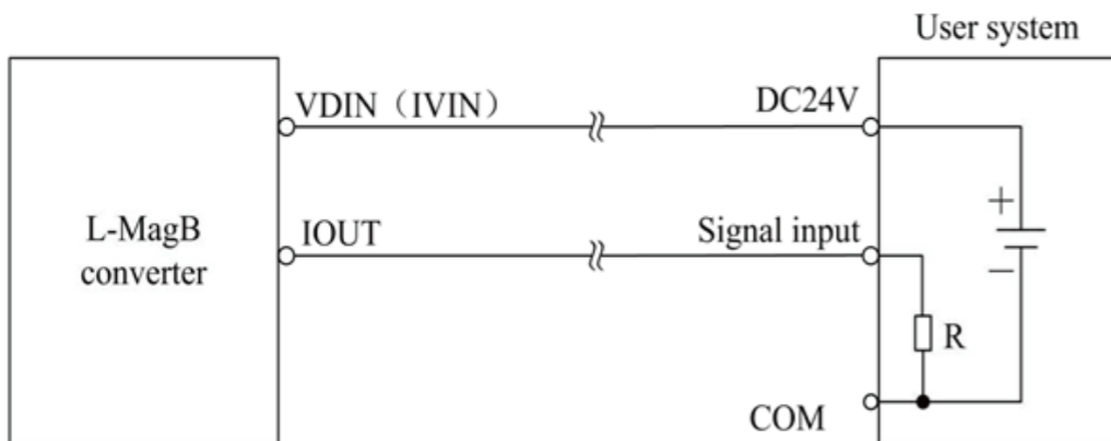
Fig.4.6 (a) L_MagB two connection
