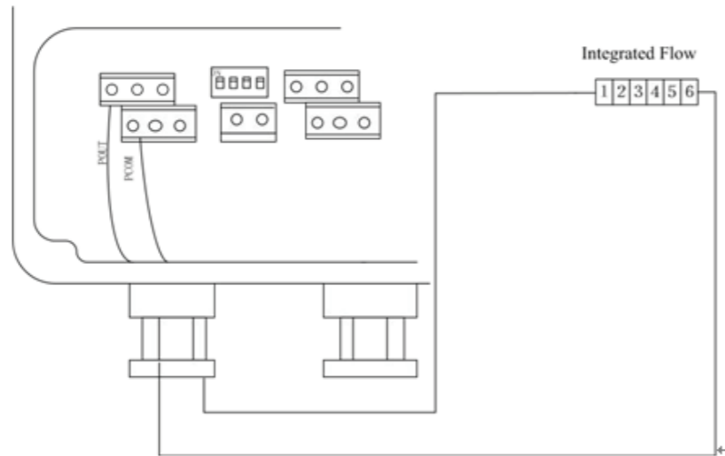
Fig.4.4 (c) Connection of electronic counter
