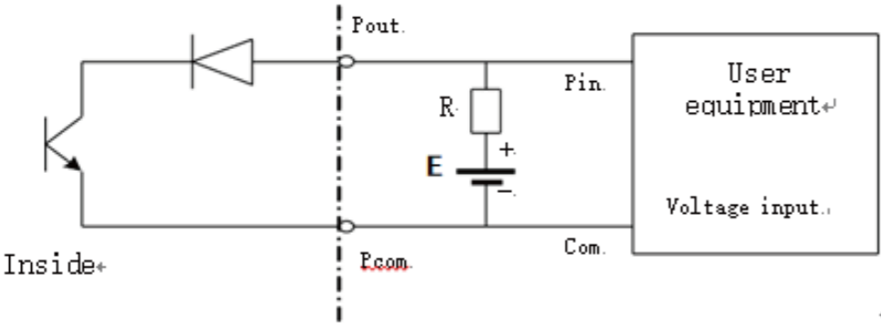
Fig.4.5(a) The connection of digital voltage output
