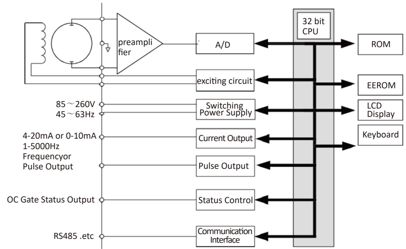
Fig.2. 1 Structure Of Converter's Circuit
