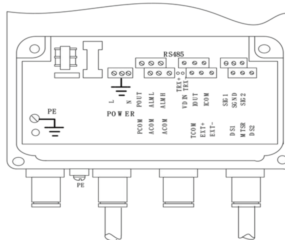
Fig.4.3 (a) Connectors for 211B
