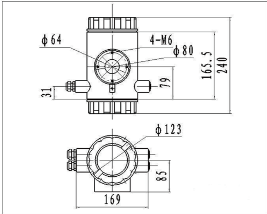
Fig.1 Exterior size of the integrated Circular shells
