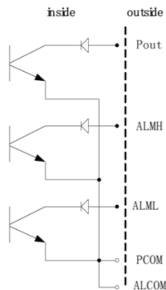
Fig.4.4 (e) Connection of OC gate
