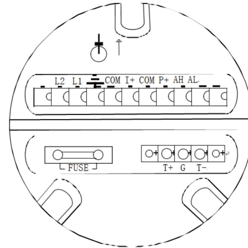
Fig.4.3(c) Connectors in circular model
