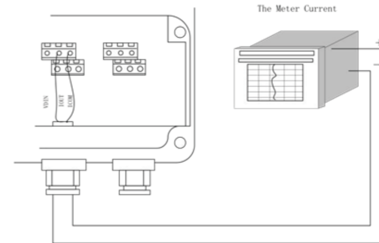
Fig.4.4 (a) Output current circuit
