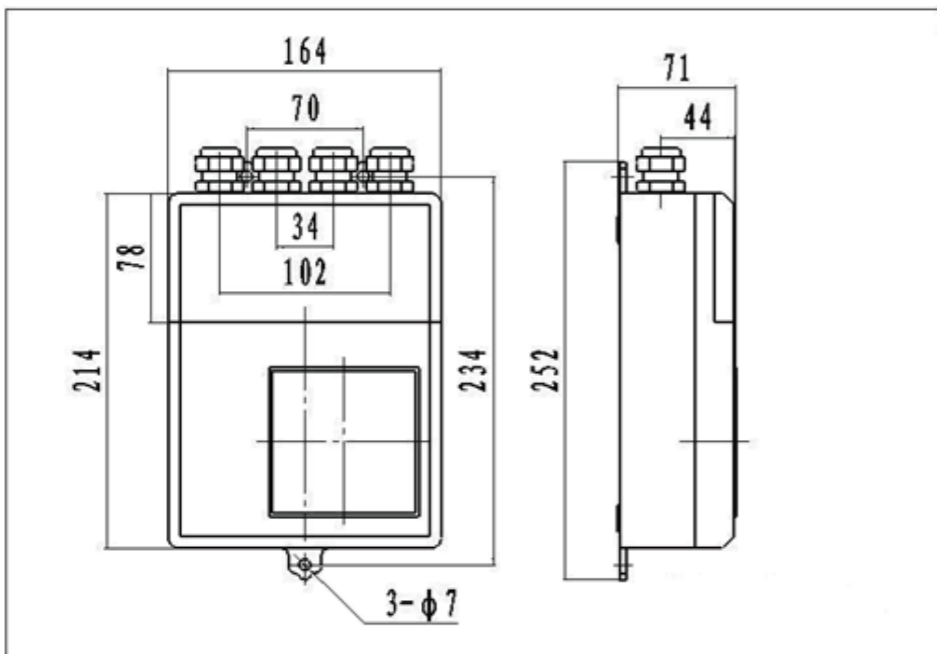
Fig.2 Exterior size of the split squared shells
